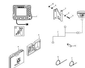
ETB-003478, Isobus Amatron 3
