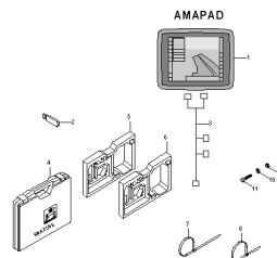
ETB-003480, Isobus Amapad
